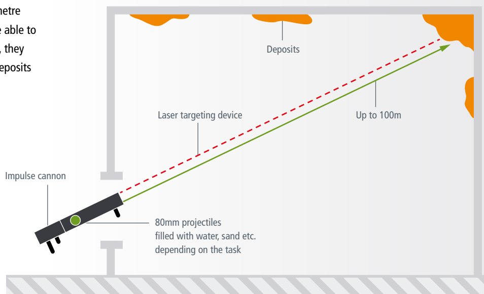
How our industrial cannon works
